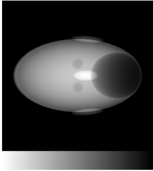
(a) 2次元投影 p(X, Z, \beta = 0)
