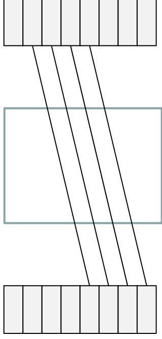
(b) Oblique projection
