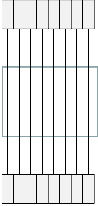
(a) Direct projection
